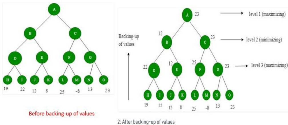
Figure 2.43 MAX-VALUE and MIN-VALUE
