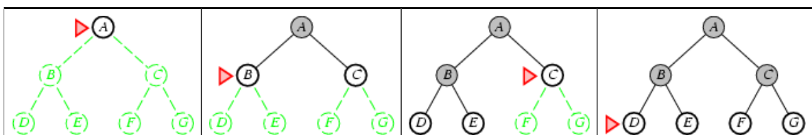
Figure 2.5 Breadth-first search on a simple binary tree. At each stage, the node to be expanded next is indicated by a marker.
